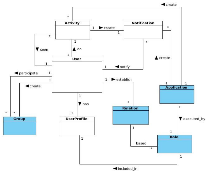
Fig. 1: Extended Social Network Model
