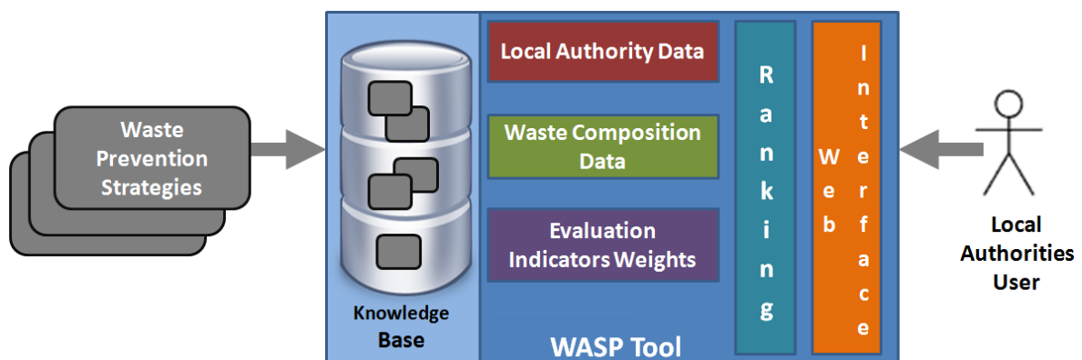
Figure1. Architecture of the WASTP Tool.
